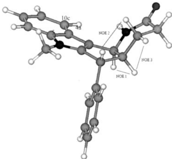
Figure 2. NOE correlations in the ^1\text{H} NMR spectrum of lactam 22a
