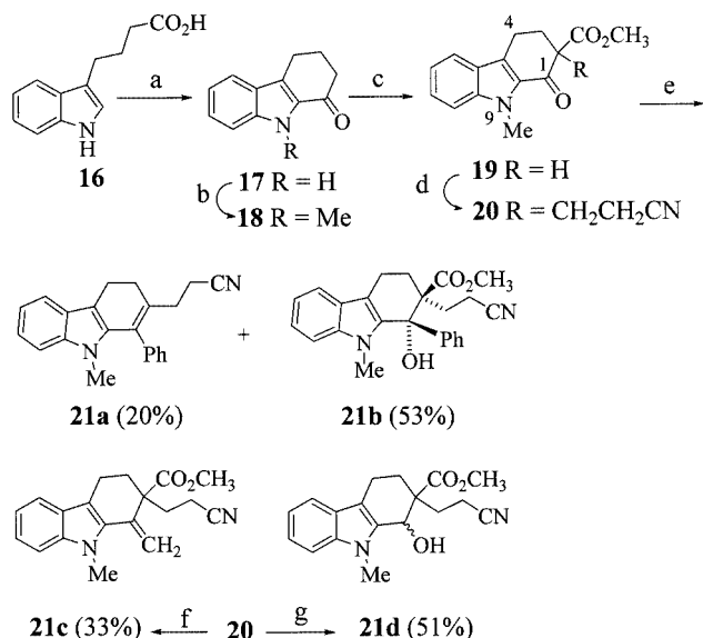
Scheme 4. Reagents and conditions: (a) PPA, toluene, 110\text{ }^{\circ}\text{C} , 85%; (b) KOH, MeI, acetone, 65%; (c) KH, (\text{CH}_3\text{O})_2\text{CO} , 150\text{ }^{\circ}\text{C} , 74%; (d) t\text{BuOK} , acrylonitrile, t\text{BuOH} , 73%; (e) \text{PhMgBr} , THF, -78\text{ }^{\circ}\text{C} ; (f) \text{MeMgBr} , THF, -78\text{ }^{\circ}\text{C} ; (g) \text{NaBH}_4 , MeOH, de = 30\%
