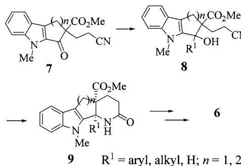
Scheme 1. Planned conversion of indole-based precursors 7 into tetracyclic ester compounds 9 [2]
