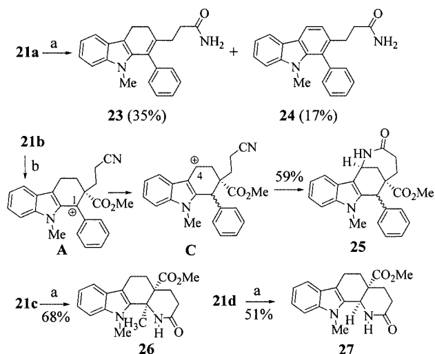
Scheme 6. Reagents and conditions: (a) \text{CH}_3\text{SO}_3\text{H} , \text{PhCl} , 100 °C; (b) \text{CH}_3\text{SO}_3\text{H} , as solvent, room temp.
