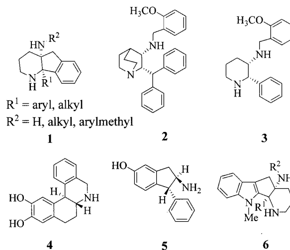
Figure 1. Structures of diamine model compounds and target compounds
