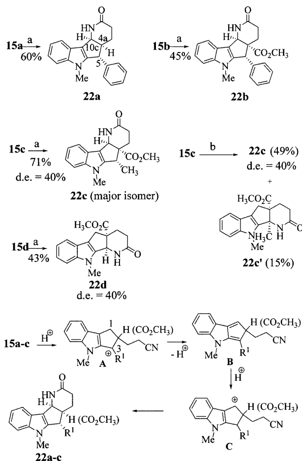
Scheme 5. Reagents and conditions: (a) \text{CH}_3\text{SO}_3\text{H} , PhCl, 100\text{ }^{\circ}\text{C} ; (b) \text{CH}_3\text{SO}_3\text{H} , as solvent, room temp.
