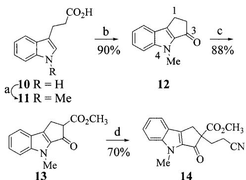
Scheme 2. Reagents and conditions: (a) (i) KOH, MeI, acetone; (ii) KOH, H 2 O, reflux; (b) PPA, toluene, 110 °C; (c) KH, (CH 3 O) 2 CO, 150 °C; (d) t BuOK, acrylonitrile, t BuOH
