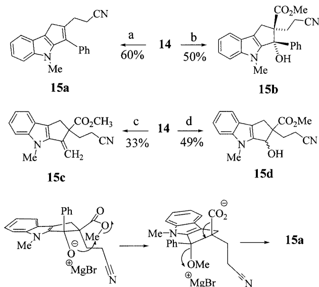
Scheme 3. Reagents and conditions: (a) PhMgBr, THF, -78 °C; (b) PhMgBr, Et 2 O, -78 °C, de = 26%; (c) MeMgBr, THF, -78 °C; (d) NaBH 4 , MeOH, phosphate buffer pH = 7, de = 12%
